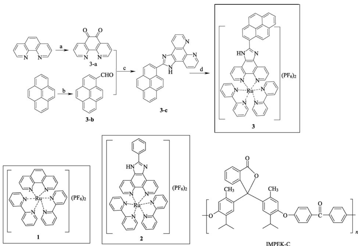
Scheme 1 The structure of complexes 1 and 2 as well as the synthesis of complex 3 . a: KBr, H 2 SO 4 /HNO 3 , 100°C, 3 h; b: POCl 3 , DMF, CHCl 3 , 60°C, 20 h; c: ammonium acetate, acetic acid, 60°C, 6 h; d: EtOH, r.t. 4 h, 2,2'-bipyridine, H 2 O, 100°C, 24 h. The molecular structure of the IMPEK-C polymer was also shown.
