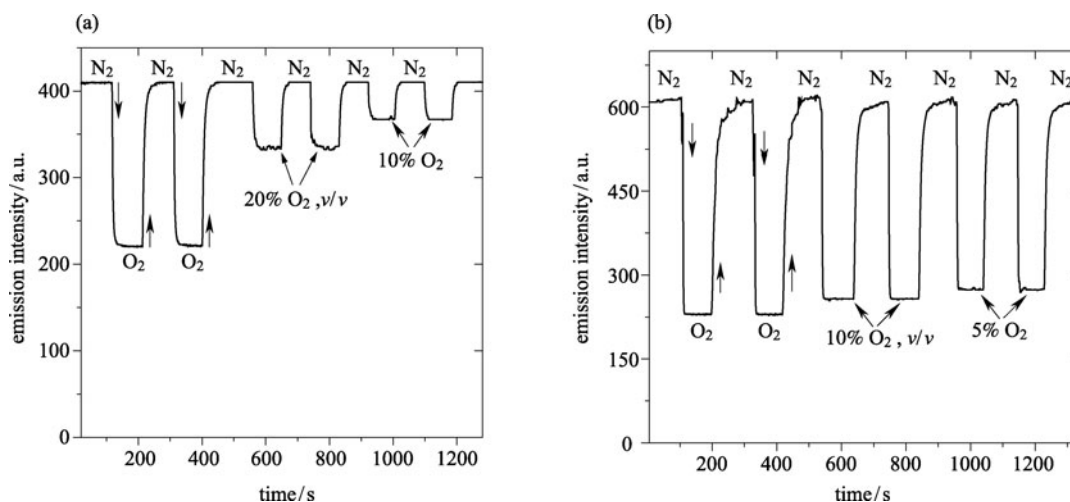
Figure 3 Phosphorescent intensity response of sensing films of the complexes 2 and 3 in IMPEK-C to O_2/N_2 saturation cycles. (a) complex 2 , \lambda_{ex}=476 nm, \lambda_{em}=593 nm; (b) complex 3 , \lambda_{ex}=478 nm, \lambda_{em}=593 nm. In order to compare the quenching properties of the films, the y axis is set from 0. Measurements were taken with home-assembled optical fiber/flow cell system.
