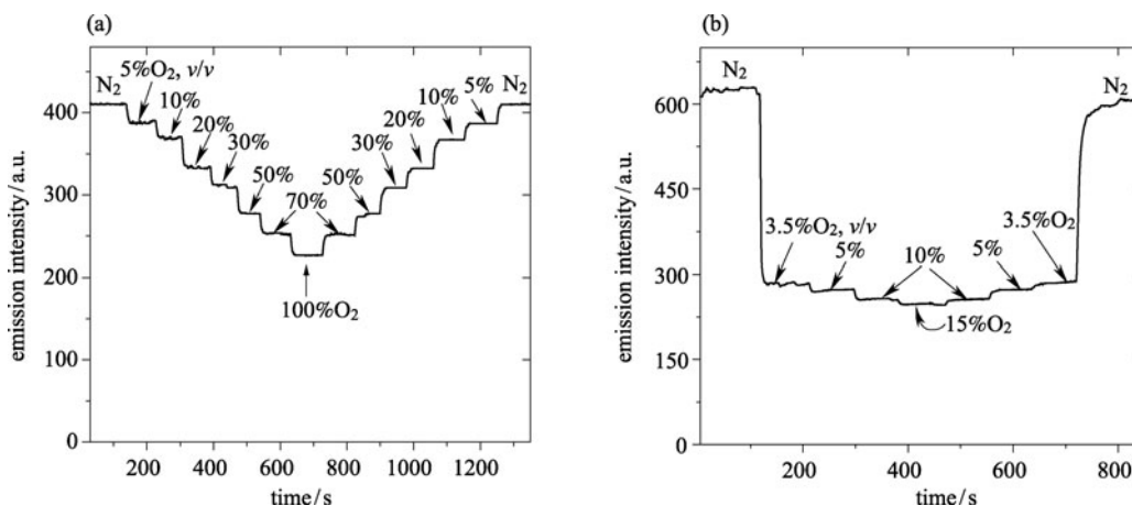
Figure 4 Phosphorescent intensity response of sensing films of the complexes in IMPEK-C to step variations of O_2 concentrations. (a) complex 2 , \lambda_{ex}=476 nm, \lambda_{em}=593 nm; (b) complex 3 , \lambda_{ex}=478 nm, \lambda_{em}=593 nm. In order to compare the quenching efficiencies of the films, the y axes are set from 0 for all the figures. Measurements were taken with home-assembled optical fiber/flow cell system. The numbers indicate the O_2 concentration in mixed O_2/N_2 gas (v/v).
