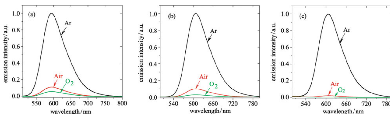
Figure 2 Room-temperature emission spectra of complexes 1 , 2 and 3 under Ar, air and O 2 atmosphere. (a) complex 1 , \lambda_{\text{ex}} = 445 \text{ nm} , (b) complex 2 , \lambda_{\text{ex}} = 457 \text{ nm} , (c) complex 3 , \lambda_{\text{ex}} = 458 \text{ nm} . Measurements were taken in 1.0 \times 10^{-5} \text{ mol} \cdot \text{L}^{-1} complexes solution in acetonitrile at 25°C.
