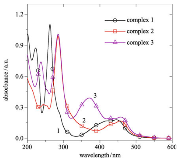
Figure 1 UV-Vis absorption spectra of Ru(II) polypyridine complexes 1 , 2 , and 3 . Measurements were carried out using 1.0 \times 10^{-5} \text{ mol} \cdot \text{L}^{-1} solution in acetonitrile at 25^\circ\text{C} .
