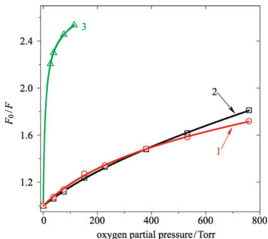
Figure 5 Oxygen sensitivity of the emission of complexes 1 , 2 and 3 . The fittings are based on the data of Figure 4 and the two-site model (Eq. (1)). The supporting polymer film of complex 1 is IMPES-C, and the supporting polymer for complexes 2 and 3 are IMPEK-C. Limited oxygen partial pressure was used for complex 3 due to the significant quenching effect.
