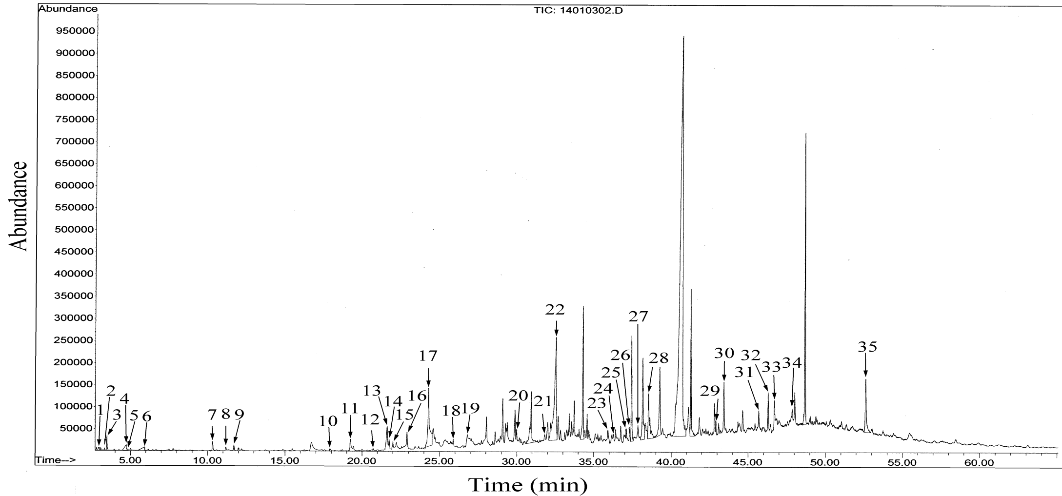
Fig. S1 GC chromatogram of the root exudates collected from fennel plant. Peaks 1 to 35 were identified by MS (see Table 1).
