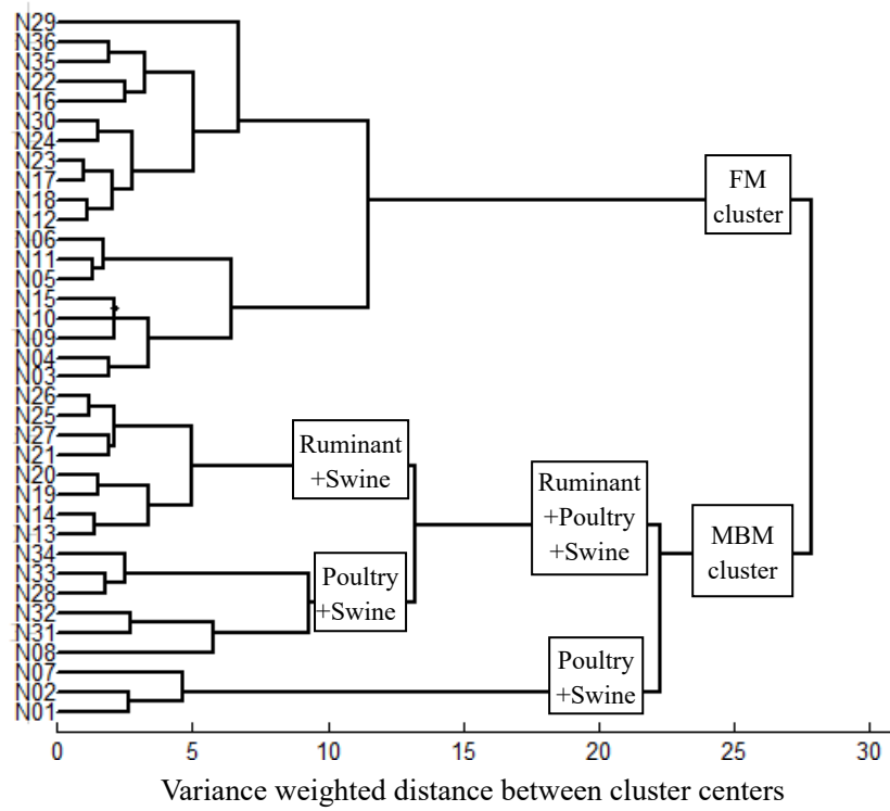
Fig. S1 Detected clusters of neurons by applying ward's method on the weights of the SOFM neurons after training. N01-N36 indicates neuron 01-neuron 36.
