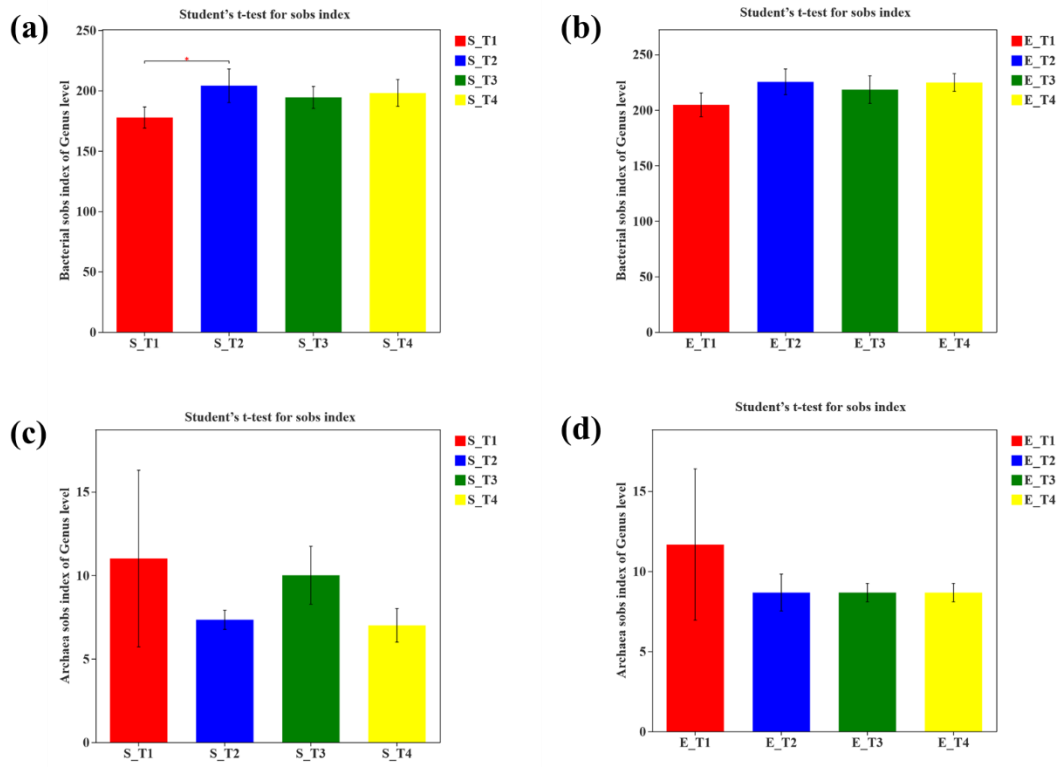
Fig. S1 Diversity index difference test chart between groups (Genus level). (a) Bacterial diversity index difference test chart between stable groups; (b) bacterial diversity index difference test chart between final groups; (c) archaea diversity index difference test chart between stable groups; (d) archaea diversity index difference test chart between final groups.
