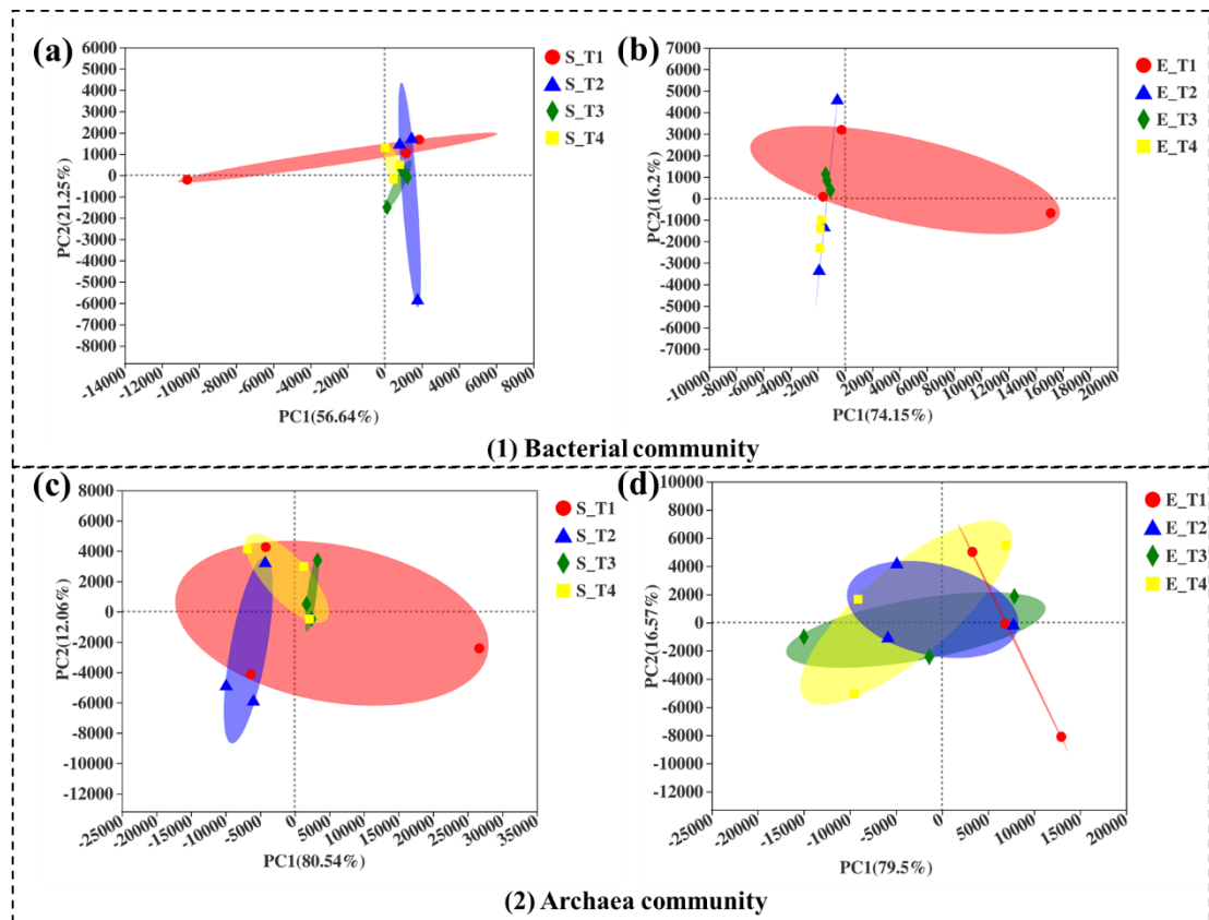
Fig. S2 Principal component analysis of microbial communities. (a) Bacterial community of stable groups; (b) bacterial community of final groups; (c) archaea community of stable groups; (d) archaea community of final groups.
