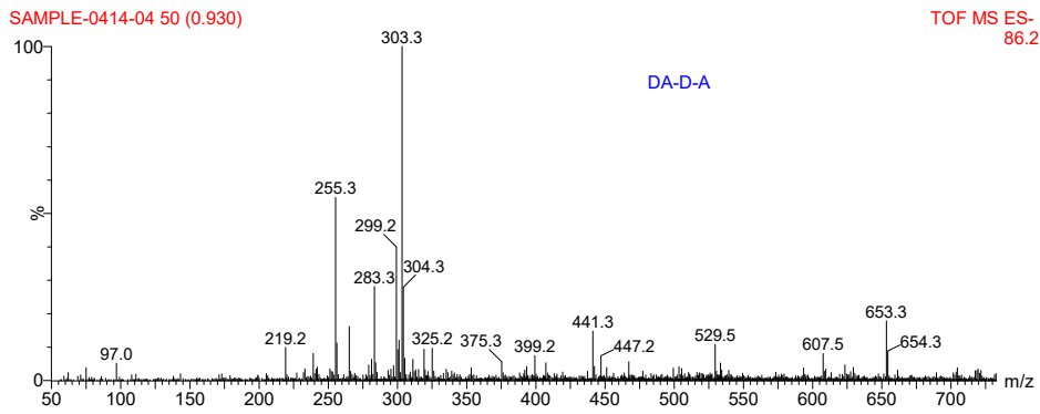
Fig. S1 The spectrum of mass spectrometer
