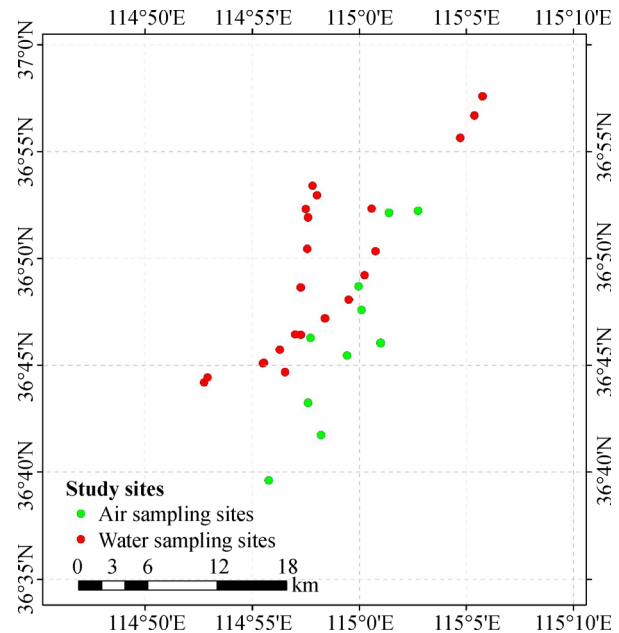
Fig. 2 Spatial distribution of surface water and ammonia sampling sites in Quzhou County.
