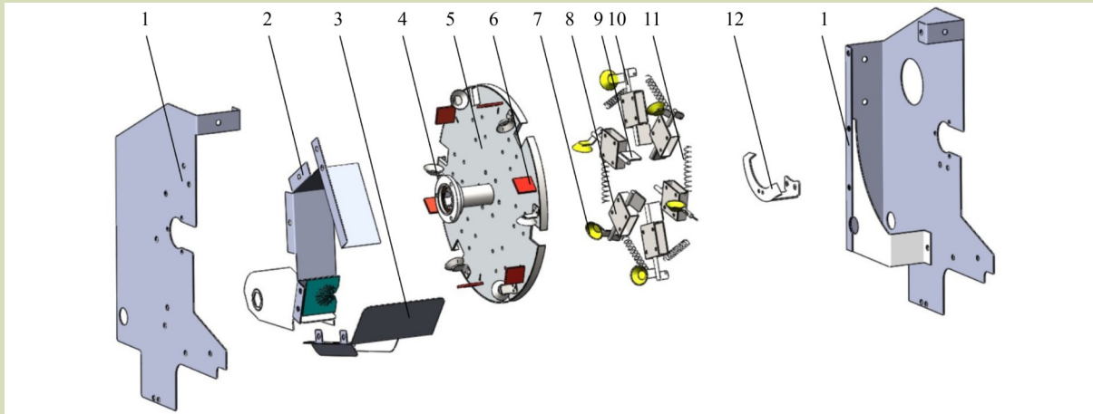
Fig. 1 Seed-metering device: 1, side plates; 2, intermediate partition; 3, falling seed guide plate; 4, seed-collection spoons; 5, seed tray; 6, seed-distribution plates; 7, pickup finger; 8, pickup finger fixing boxes; 9, finger trail clip; 10, finger pole; 11, fine-adjustment springs; and 12, control board that opened and closed the clip.
