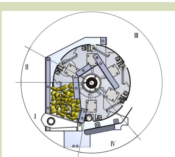
Fig. 2 Seed-metering device: I, loading area; II, clamping area, III, transfer area; and IV, delivery area.
