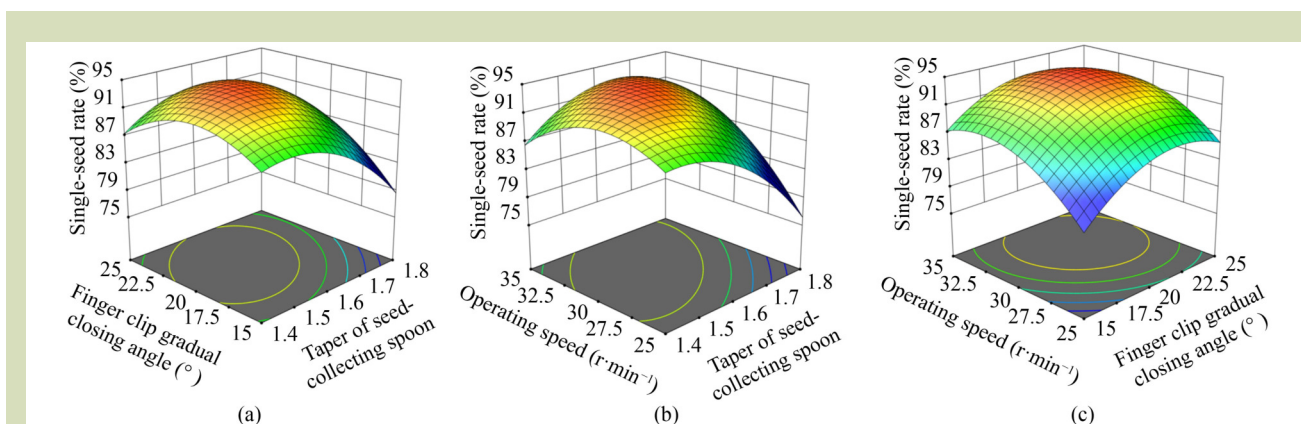
Fig. 20 Effects of interacting factors on the single-seed rate: (a) finger clip closing angle vs. taper of seed-collection spoon; (b) operation speed vs. taper of seed-collection spoon; and (c) operating speed vs. finger clip gradual closing angle.
