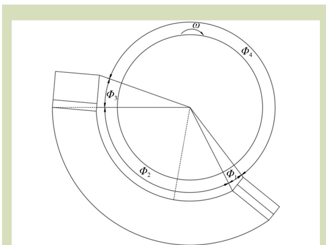
Fig. 6 Control board partitions. The finger clip gradual opening angle is denoted by \Phi_1 , the finger clip complete opening angle is denoted by \Phi_2 , the finger clip gradual closing angle is denoted by \Phi_3 and the finger clip complete closing angle is denoted by \Phi_4 .
