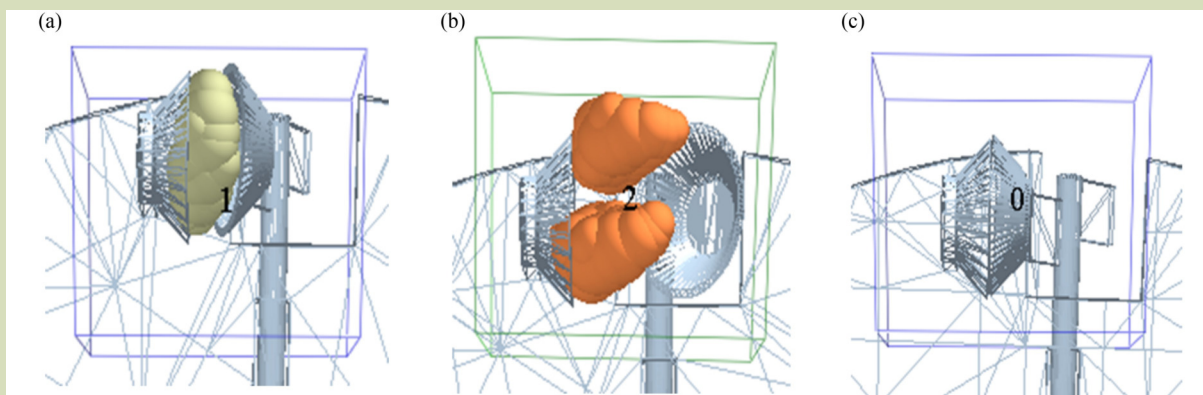
Fig. 14 Three loading states exhibited during the simulation process: (a) single-seed; (b) multiple-seed; and (c) no seed (empty).
