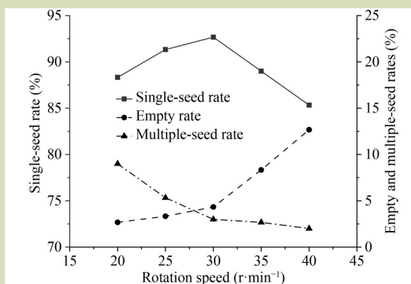
Fig. 19 Relationship between evaluation indicators and different rotation speeds of the seed tray.
