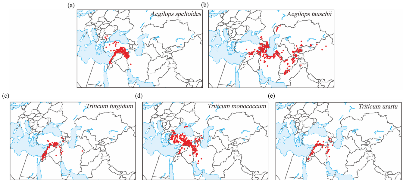
Fig. 2 Distribution of the allied species of wheat (source from GBIF datasets [32] ) (审图号: GS (2020) 7209号)
