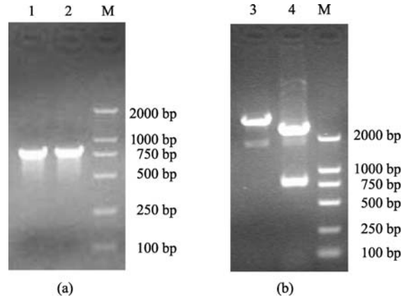
Fig. 2 Identification of the recombinant plasmid pMD-M
