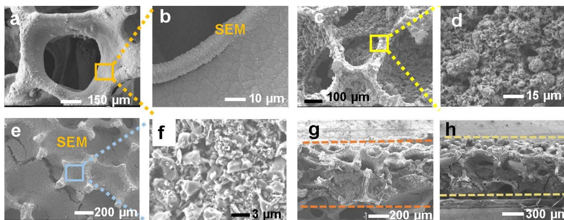
Figure 1 (a-b): SEM images of Al foam@C; (c-d): SEM images of Al foam@G; (e-f): SEM images of Al foam@C filled with MC; Cross-section SEM images of Al foam@C filled with MC (g) and Al foam@G filled with MC (h). (color on line)
