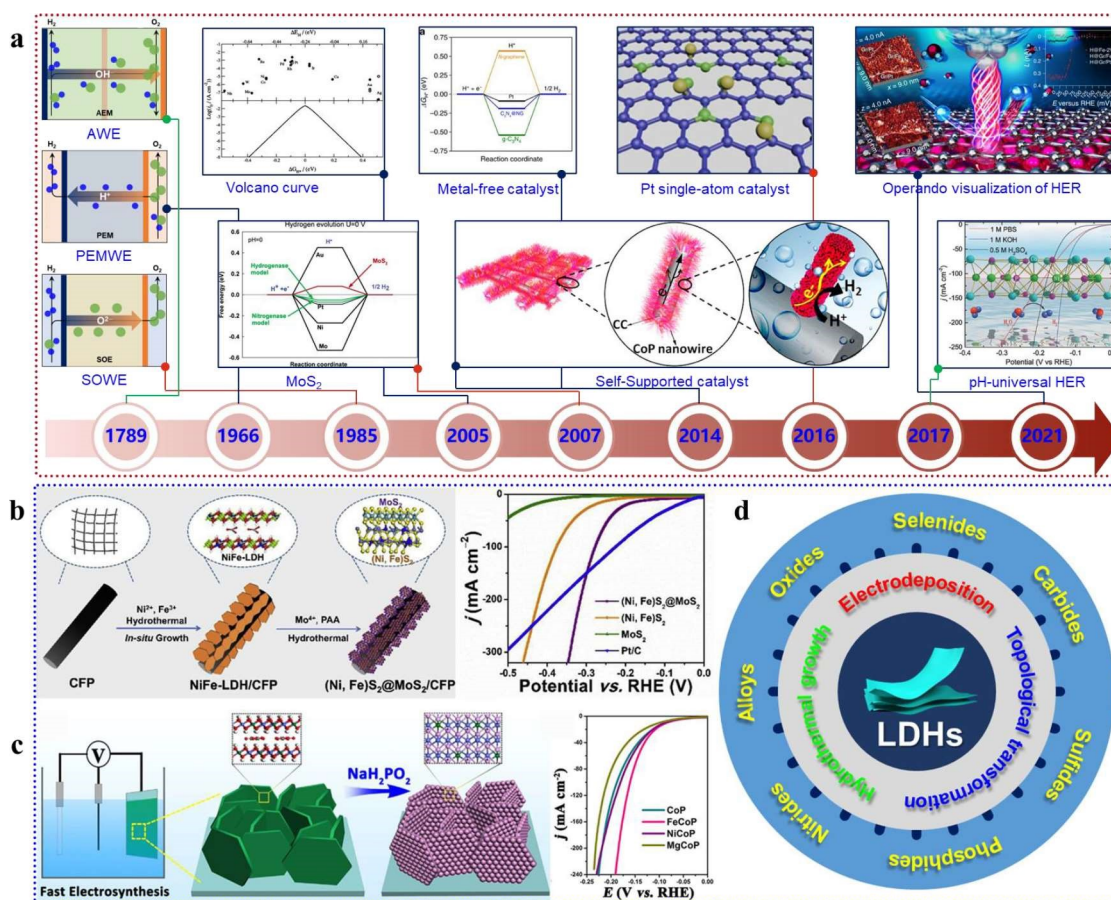
Figure 3 (a) Timeline of recent developments for water electrolysis. (b) Illustration and HER performance of (\text{Ni, Fe})\text{S}_2@\text{MoS}_2 [53] . Reproduced with permission of Ref. 53, copyright Elsevier. (c) Illustration and HER performance of FeCoP [54] . Reproduced with permission of Ref. 54, copyright Elsevier. (d) Schematic presentation of LDHs-derived materials. (color on line)
