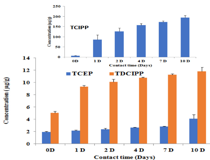
Figure 3. Average concentrations ( \mu\text{g/g} ) of CL-OPEs in dust over contact time.
