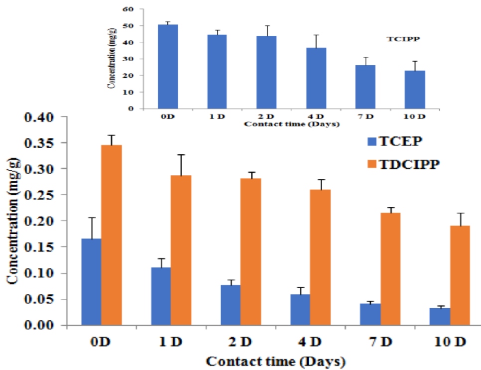
Figure 2. Average concentrations (mg/g) of CI-OPEs in fabric over contact time (y-error bars denotes 1 standard deviation).
