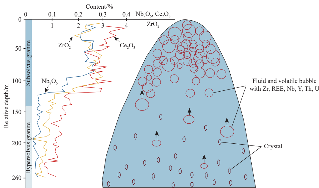
Fig. 4. Model diagram of upward migration of Zr, Nb, REE and other elements (after Yang WB et al., 2014).
