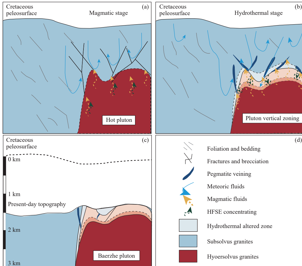
Fig. 5. Mineralization model map of Baerzhe Nb-Zr-REE deposit (after Yang WB et al., 2020). a—During the magmatic stage, granite crystals contain volatile elements such as F and Cl, which form complexes with HFSE to facilitate melting and upward migration; b—hydrothermal fluid rich in HFSE interact with groundmass resulting in alteration and precipitation of zircon. c—present Baerzhe Nb-Zr-REE deposit.
