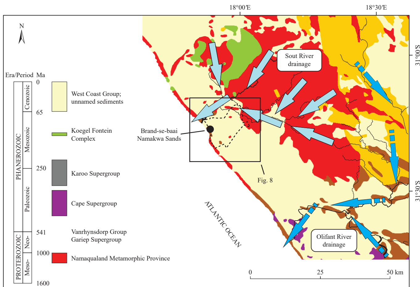
Fig. 9. Most likely provenance areas for the Namakwa Sands deposit. The schematic arrows delineate the sediment transport pathway from the Namakwa Sands provenance through the Sout-Ofiants fluvial system to its terminal depocenter in the Atlantic Ocean basin (modified from Philander C and Rozendaal A, 2015a).
