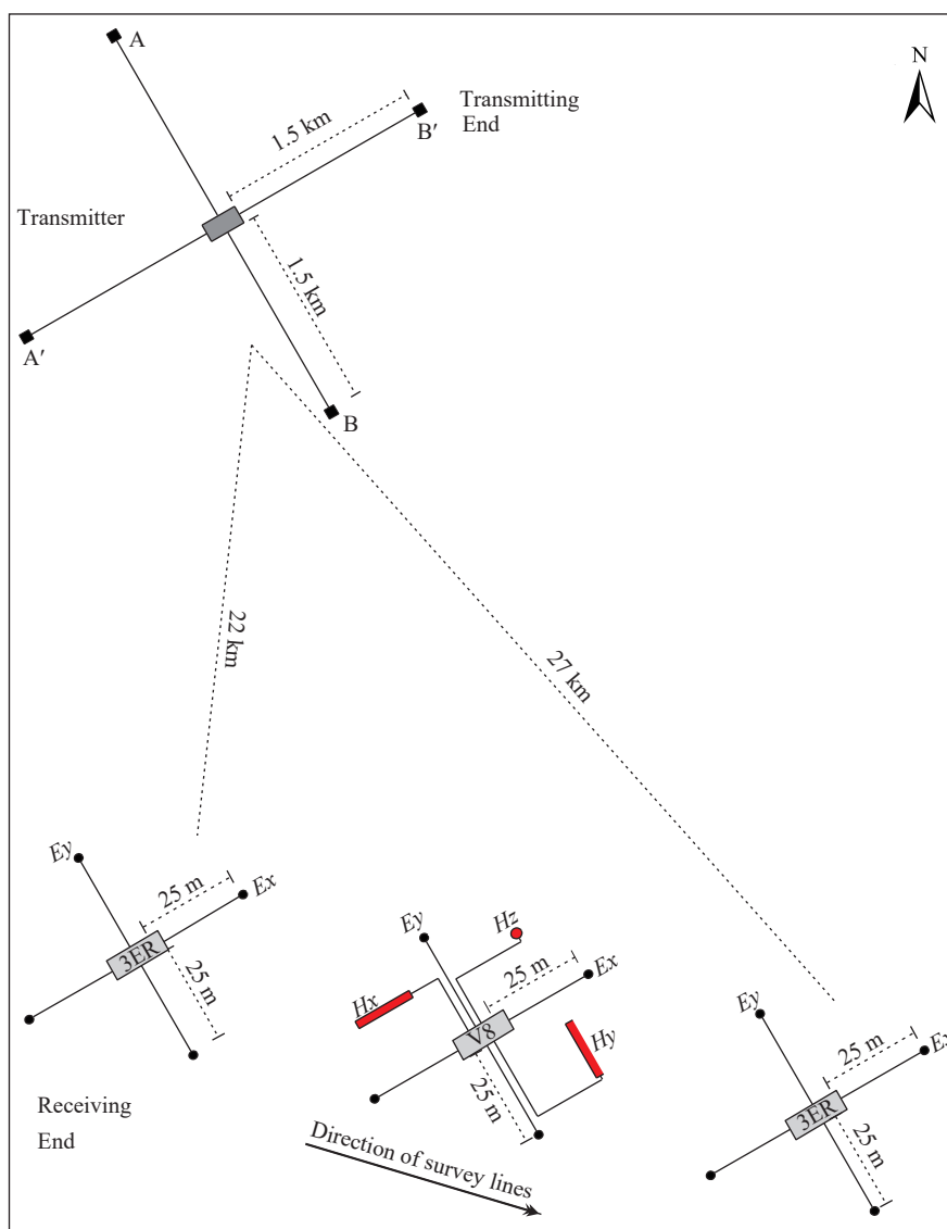
Fig. 7. Diagram of source and receiving devices of the high-power tensor CSAMT applied in the Jiama porphyry copper deposit..
