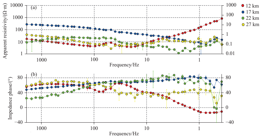
Fig. 3. Comparison of test curves in the case of different transmitter-receiver distances. a–Resistivity curves; b–phase curves.
