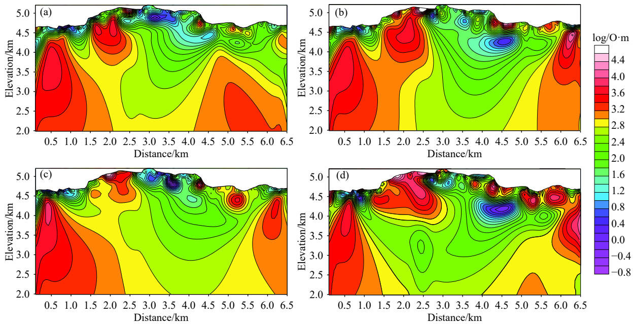
Fig. 10. 2D inversion results of four sets of high-power tensor CSAMT data along section BB'. a–EW-direction transmitting and NS-direction receiving; b–EW-direction transmitting and EW-direction receiving; c–NS-direction transmitting and NS-direction receiving; d–NS-direction transmitting and EW-direction receiving.
