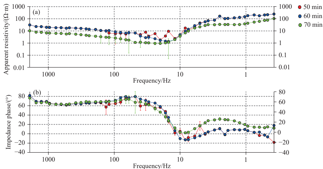
Fig. 6. Comparison of test curves in the case of different observation duration. a–resistivity curves; b–phase curves.
