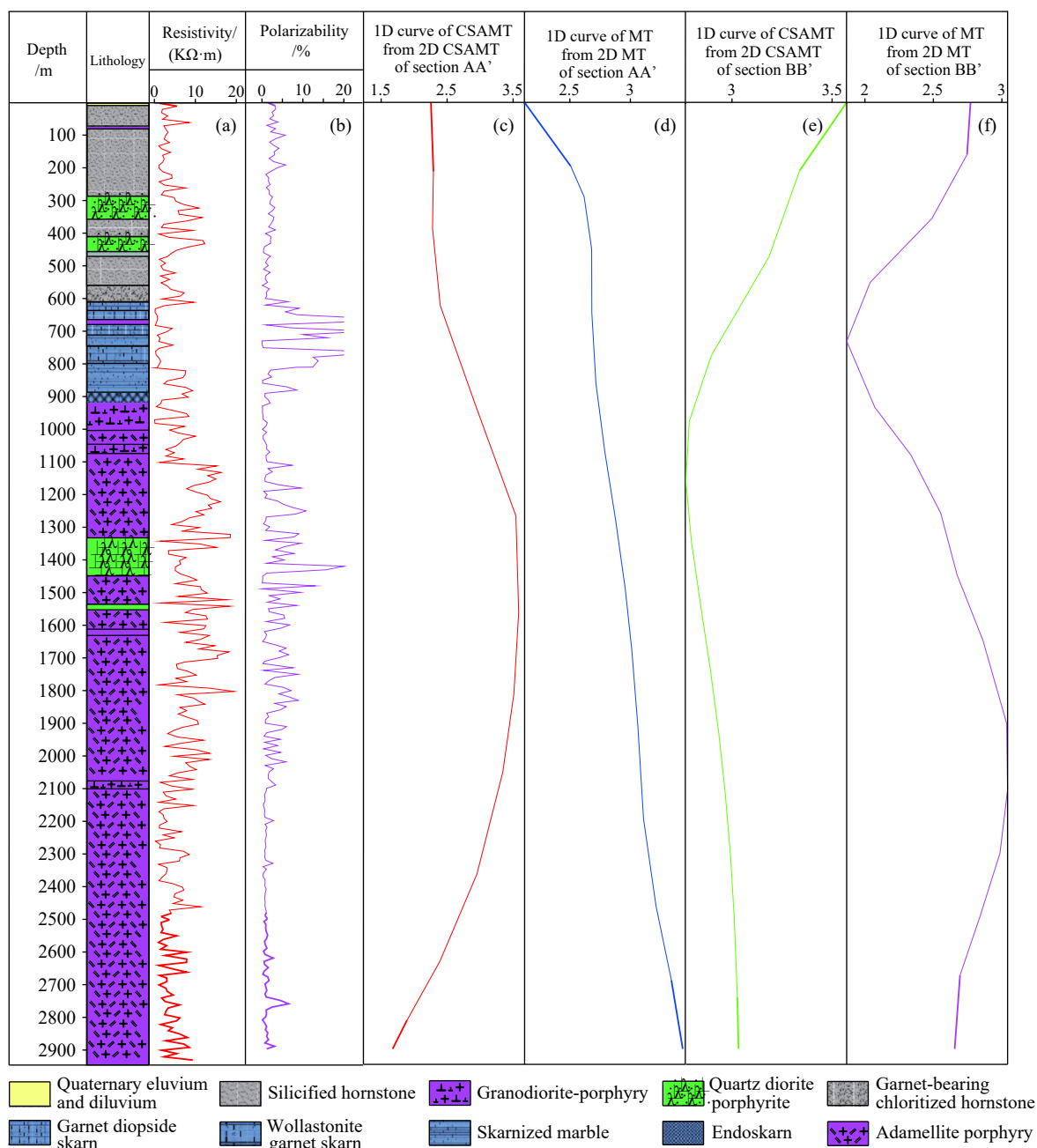
Fig. 12. Histogram and curves obtained from core specimen measurement of JMKZ borehole, and inverted resistivity variation across JMKZ from MT and CSAMT of sections AA' and BB' in Fig. 11. a–measured resistivity in JMKZ Borehole; b–measured polarizability in JMKZ Borehole; c–inverted 1D CSAMT curve of section AA'; d–inverted 1D MT curve of section AA'; e–inverted 1D CSAMT curve of section BB'; f–inverted 1D MT curve of section BB'. Those location for (c), (d), (e), and (f) see successively (a), (b), (c) and (d) in Fig. 11.
