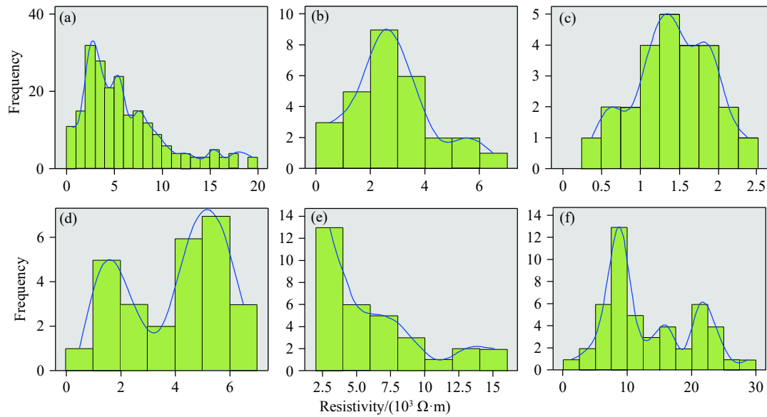
Fig. 8. Histograms for resistivity measurement of main rocks in the Jiama porphyry copper deposit. a–hornstone; b–silicified hornstone; c–skarn; d–limestone; e–quartz diorite porphyrite; f–granodiorite porphyry.
