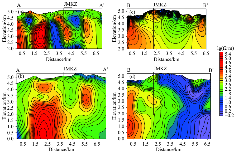
Fig. 11. Comparison of 2D inversion results of tensor CSAMT and MT data of sections AA' and BB'. a–2D CSAMT inversion results of section AA'; b–2D MT inversion results of section AA'; c–2D CSAMT inversion results of section BB'; d–2D MT inversion results of section BB'; JMKZ is a scientific borehole with a depth of 3000 m (see Fig. 1 for its location). Vertical variation of resistivity along JMKZ borehole see Fig. 12.
