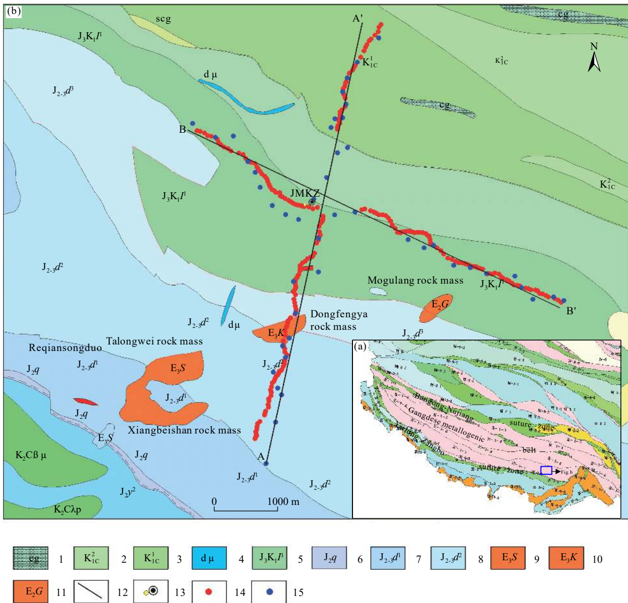
Fig. 1. Geologic map of the Jiama porphyry copper deposit and the location of research section. a—geotectonic outline map of Tibet; b—geologic map of the Jiama porphyry copper deposit (1:50000). 1—glutenite; 2—Upper member of Chumulong Formation; 3—Lower member of Chumulong Formation; 4—diorite porphyrite dike; 5—Linbuzong Formation; 6—Quesangwenquan Formation; 7—Lower member of Duodigou Formation; 8—Upper member of Duodigou Formation; 9—biotite-hornblende tonalite in Shagelang Unit; 10—adamellite porphyry in Kagazhai Unit; 11—biotite monzogranite in Guoqinglang Unit; 12—research section; 13—location of scientific borehole JMKZ with a depth of 3000 m; 14—CSAMT measurement point; 15—MT measurement point.
