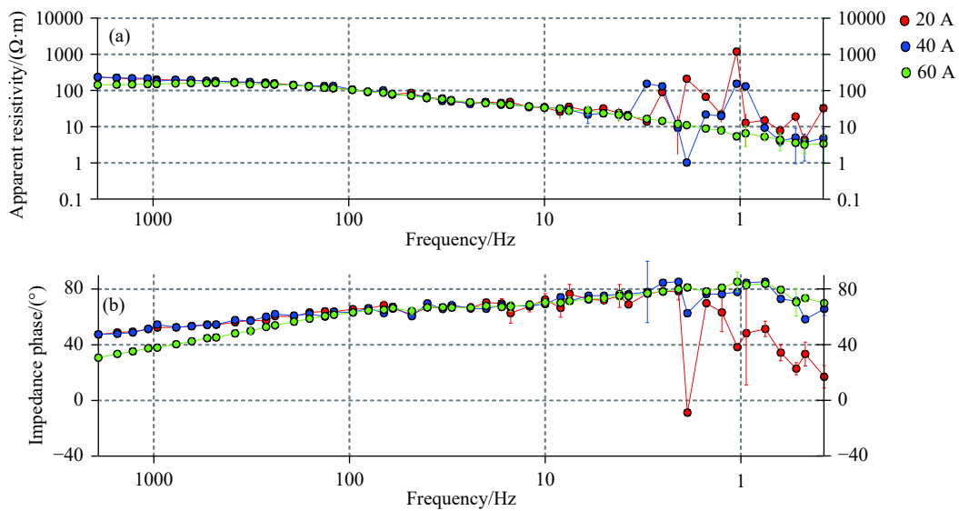
Fig. 4. Comparison of test curves in the case of different emission currents. a–Resistivity curve; b–phase curve.
