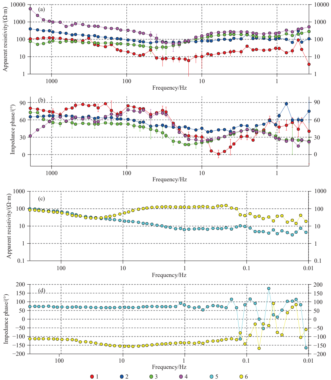
Fig. 9. Comparison of CSAMT curves collected in the case of different transmitting and receiving directions; a–CSAMT resistivity curves collected in the case of different transmitting and receiving directions; b–CSAMT phase curves collected in the case of different transmitting and receiving directions; c–MT resistivity curves; d–MT phase curves. 1–CSAMT curve collected in the case of EW-direction transmitting and NS-direction receiving; 2–CSAMT curve collected in the case of EW-direction transmitting and EW-direction receiving; 3–CSAMT curve collected in the case of NS-direction transmitting and NS-direction receiving; 4–CSAMT curve collected in the case of NS-direction transmitting and EW-direction receiving; 5–MT curve collected in the case of xy direction; 6–MT curve collected in the case of Yx direction.
