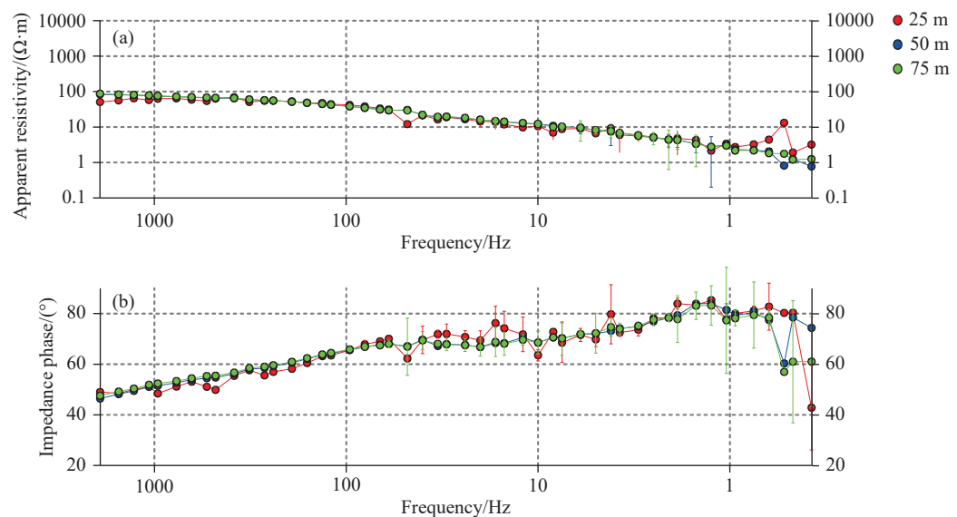
Fig. 5. Comparison of test curves in the case of different MN electrode spacing. a–Resistivity curves; b–phase curves.
