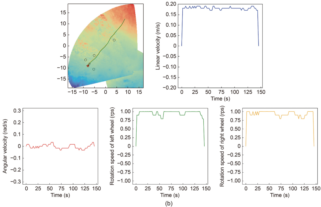
Fig. 17. (a) The result of autonomous navigation test 1 on lunar terrain. (b) The result of autonomous navigation test 2 on lunar terrain.
