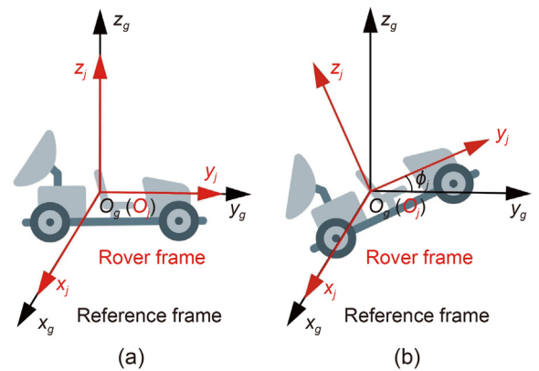
Fig. 3. (a) Reference and rover frames when slope = 0. (b) Reference and rover frames when slope = \phi_j .
