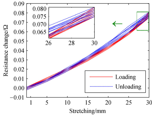
Fig. 8 Resistance performance of the soft curvature sensor under loading and unloading conditions.
