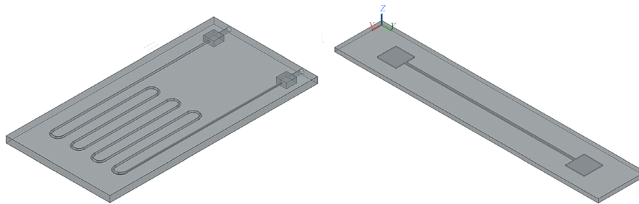
Fig. 2 Comparison of the structural design of serpentine and linear microchannels.
