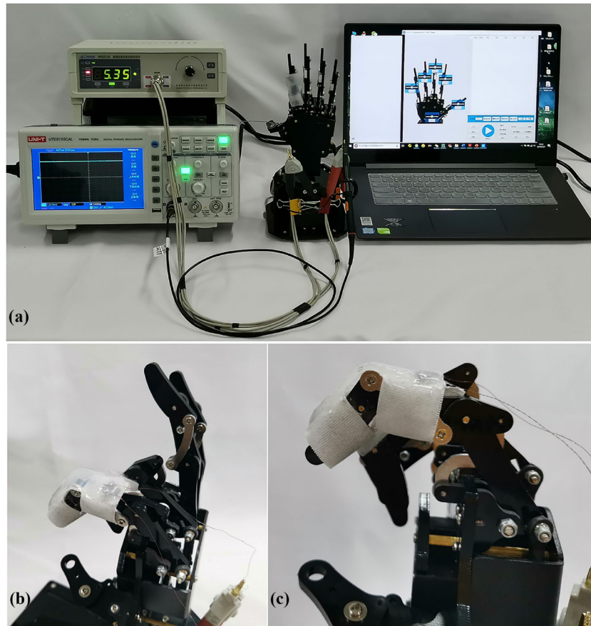
Fig. 9 Experimental platform for measuring mechanical fingers with the soft curvature sensor: (a) Experimental platform, (b) large bending angle, and (c) small bending angle.
