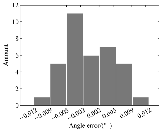
Fig. 13 Histogram of the deviation between theoretical and experimental \Delta R .
