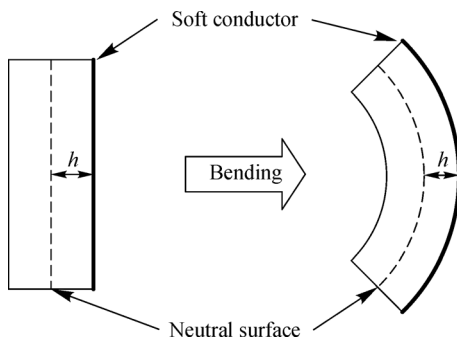
Fig. 1 Schematic of elastomer bending.
