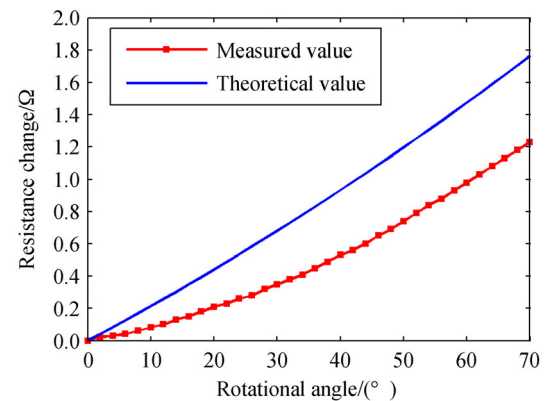
Fig. 11 Performance of the soft curvature sensor when the mechanical finger rotates.
