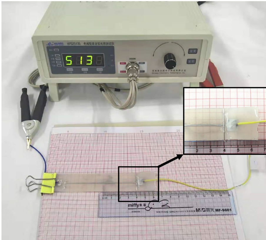
Fig. 5 Experimental platform for the stretching of a soft curvature sensor.
