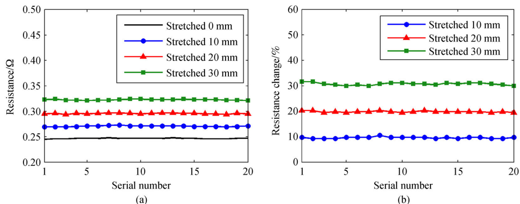
Fig. 7 Resistance performance under different stretching lengths for repeated experiments: (a) Stretched by 10, 20, and 30 mm; (b) comparison of the stretched sensor.
