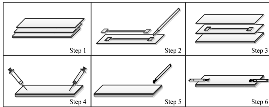
Fig. 4 Production of a soft curvature sensor.
