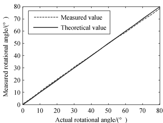
Fig. 14 Comparison of the measured rotational angle and theoretical values for repeated experiments.
