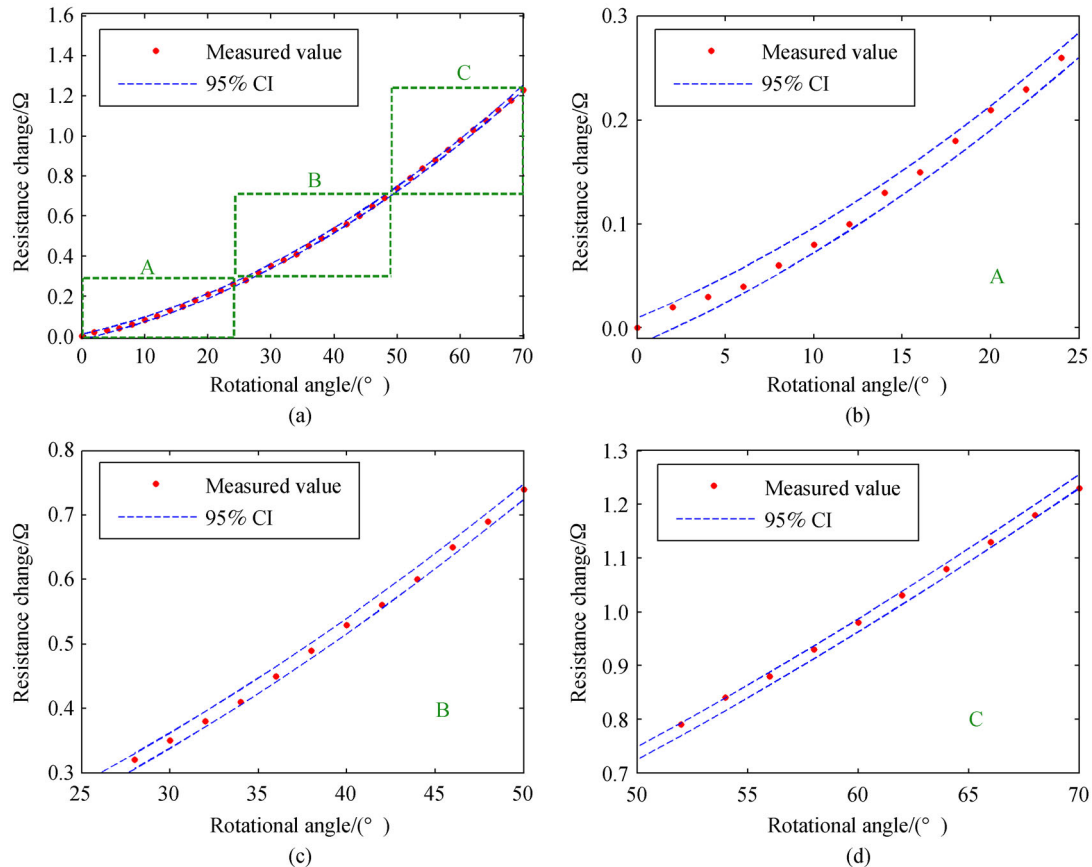
Fig. 12 Distribution of resistance changes of the soft curvature sensor versus the rotational angle of the mechanical finger: (a) Global curve; curve segments of (b) A, (c) B, and (d) C noted in (a).
