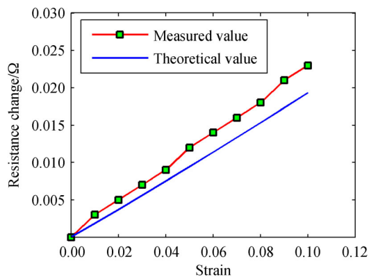
Fig. 6 Resistance change in the soft curvature sensor when stretched by 10 mm (strain: 11.2%).
