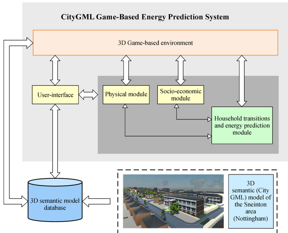
Fig. 1 Architecture of EvoEnergy.
