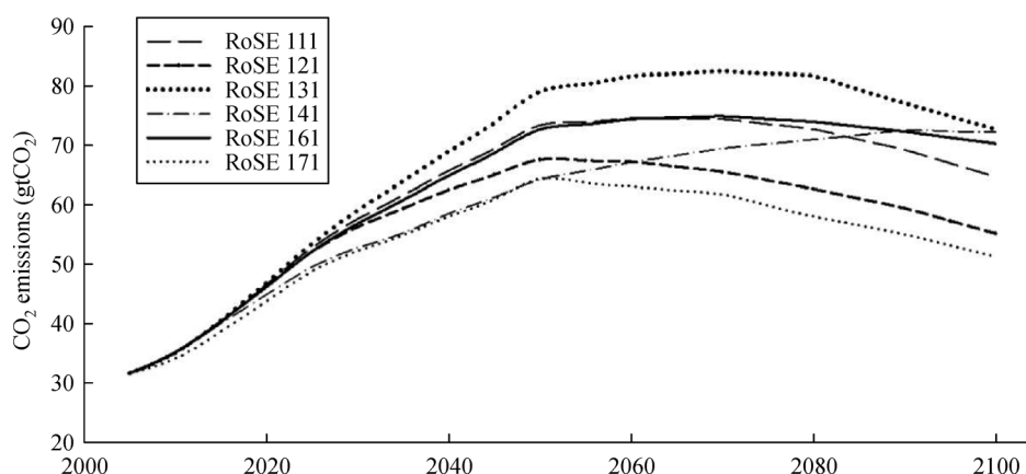
Fig. 4 CO 2 emissions in six global BAU scenarios
