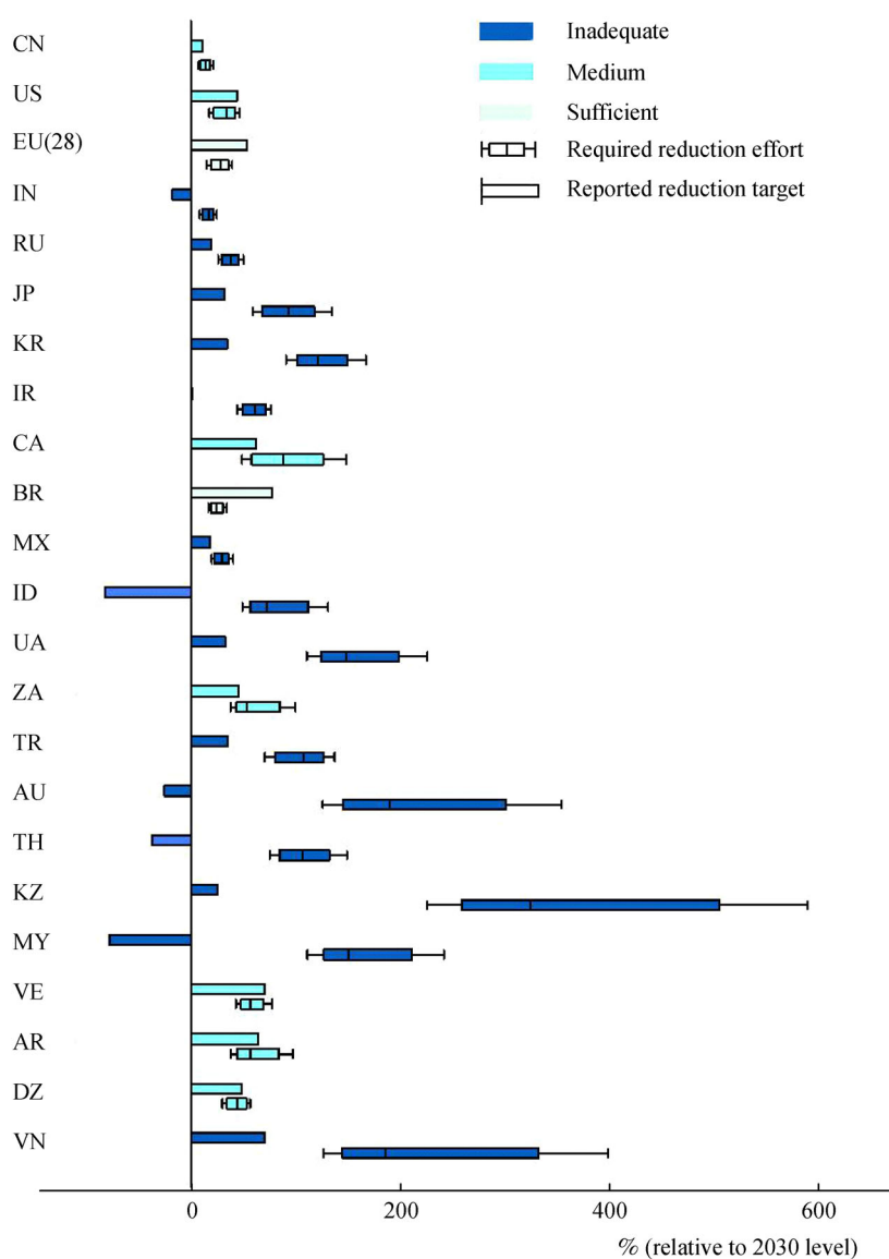
Fig. 7 Assessment result (top-down in descending order of emission shares in 2012)
